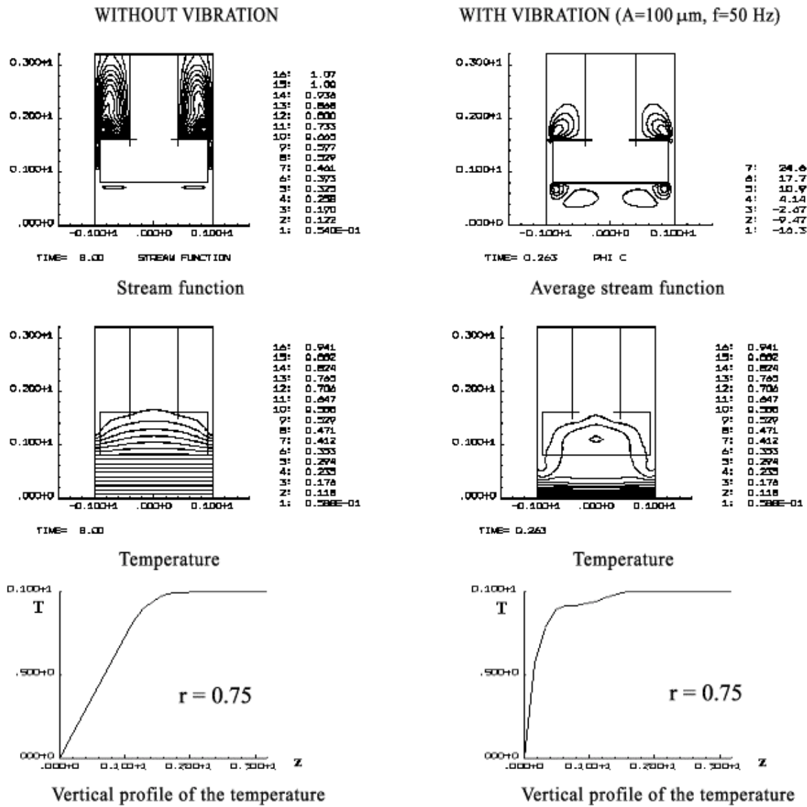
Fig.4 Influence of vibrations on a temperature boundary layer at front of a crystallization ( Gr=2.1 \cdot 10^6 , Pr=5.43 , H/R=3.2 )
