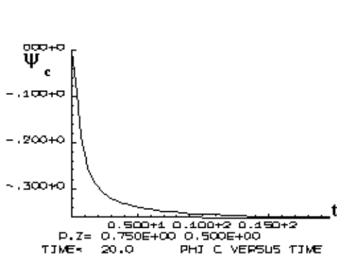
c) Change of an average stream function on time
